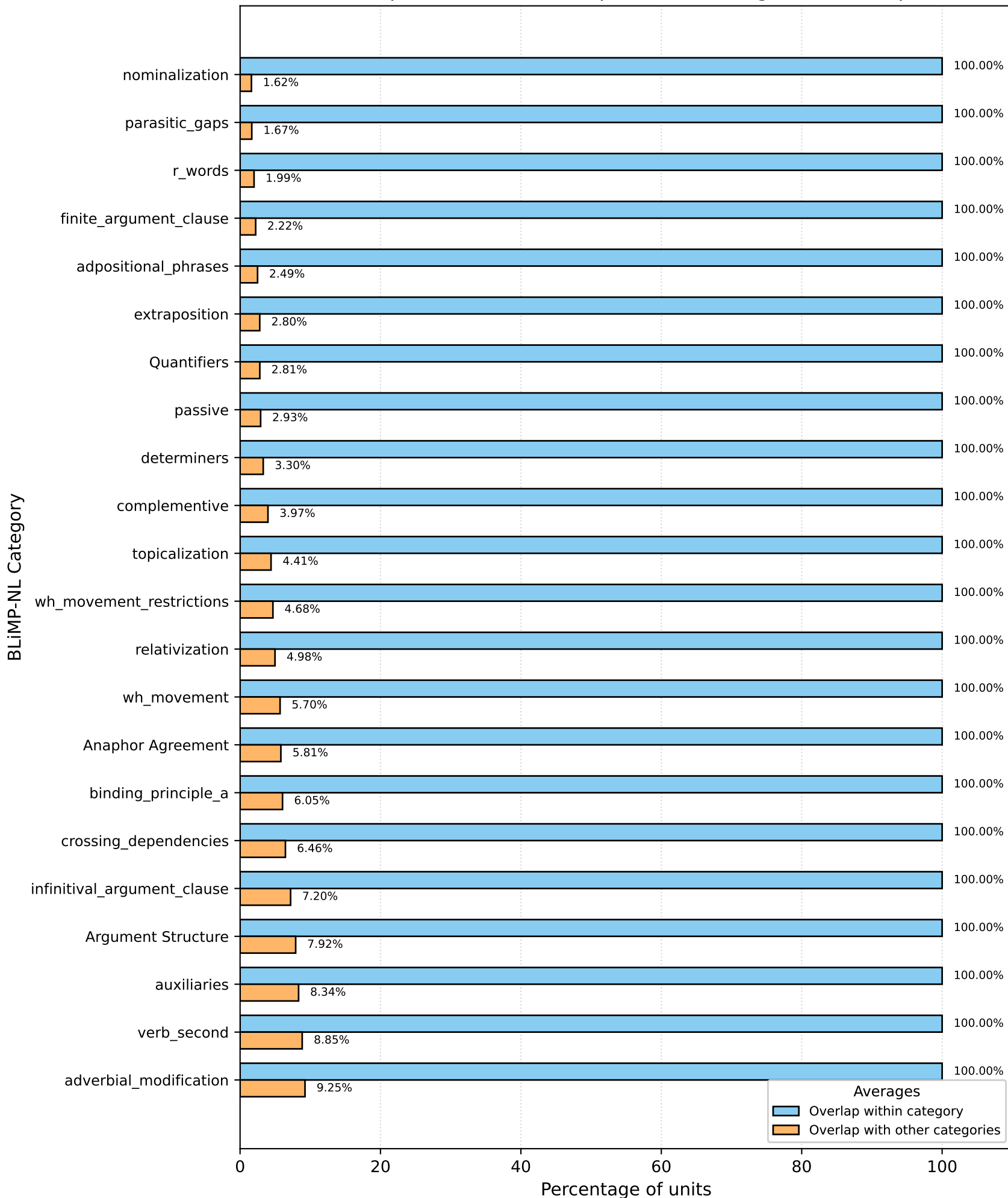
Cross-phenomenon overlap in BLiMP-NL (gemma-3-4b-pt)
